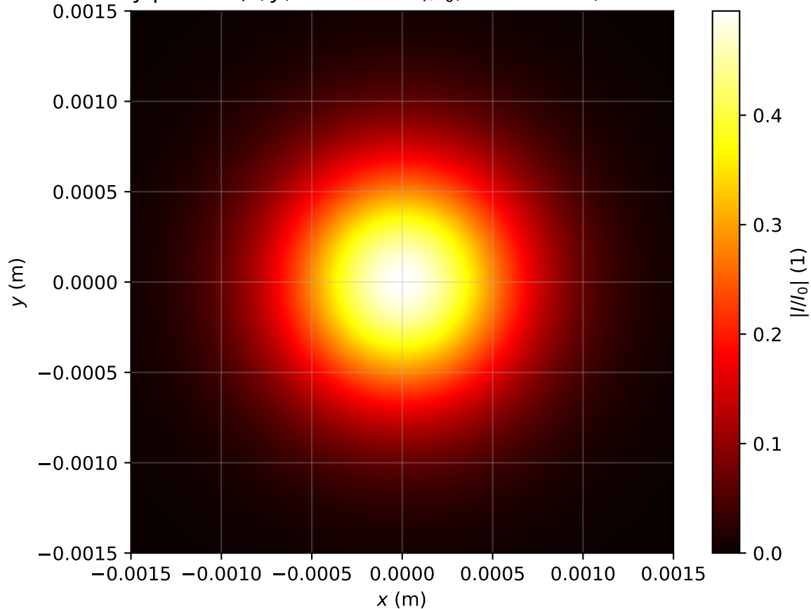
Intensity profile I(x, y, z = 2.946m)/I_0 , \text{Pin}=0.4\text{Pcr} , artificial time
